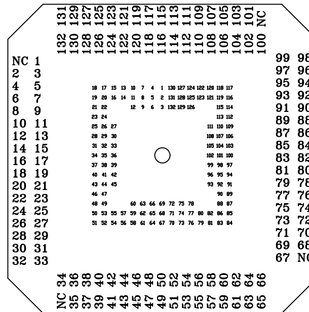
PIN #1 CORNER
