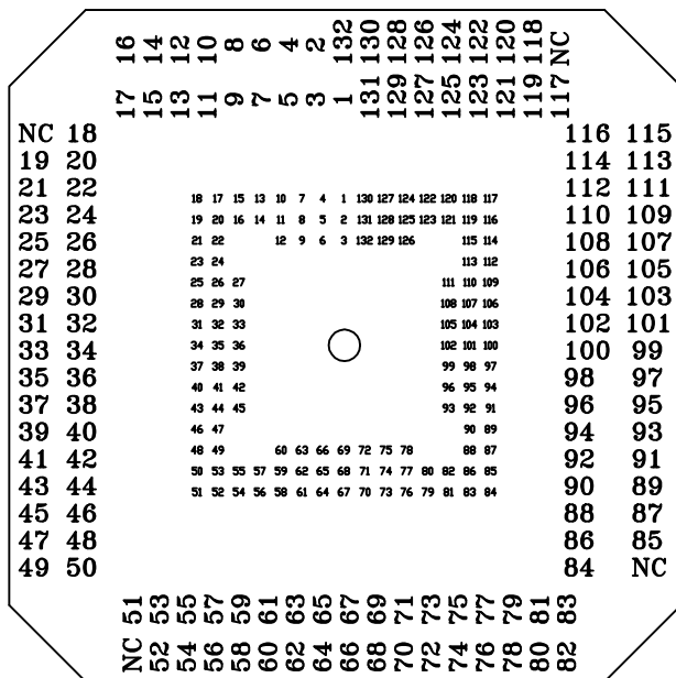
PIN #1 CENTER
