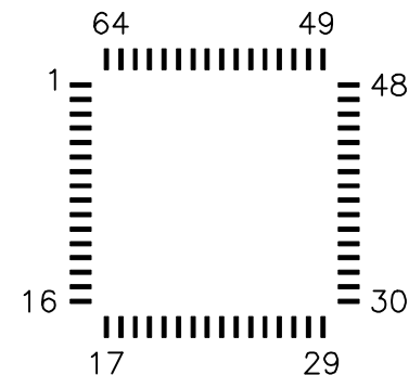
PIN MAP
